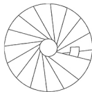
E.L.I.C.A. Diameter 210 cm; Riser: 17 cm ; Price single step: 220 Euro
